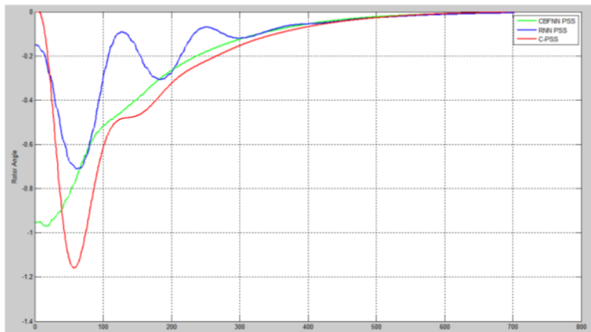
Fig. 8. Rotor Angle Comparison
