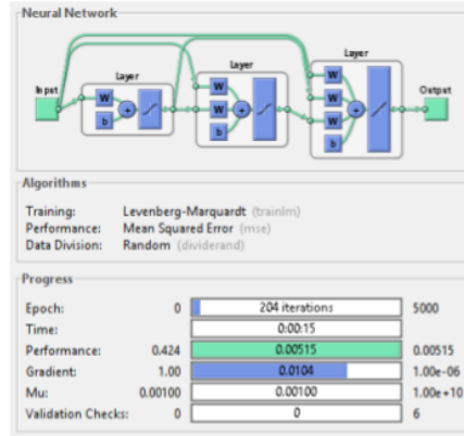
Fig. 6. Training CFBNN
