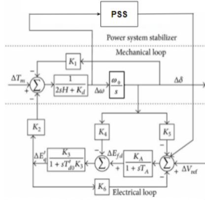
Fig. 5. Single Machine Block Diagram.
