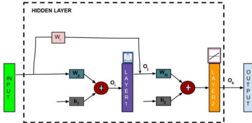
Fig. 3. Cascade Forward Backpropagation Neural Network Architecture.
